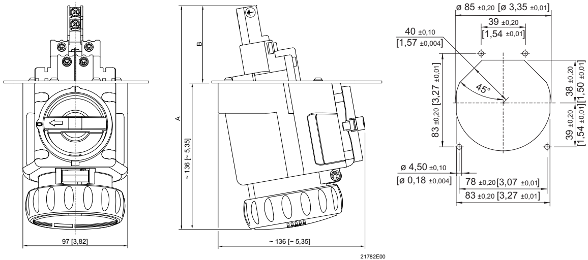
8570/25-4.. and 8570/25-5.. SolConeX flange socket
