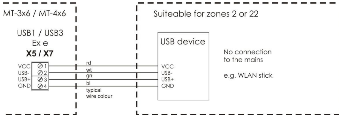
Connection diagram type 1
