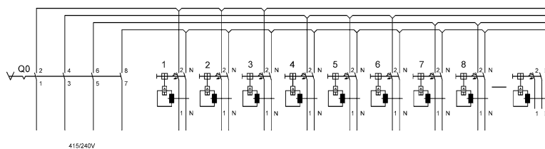
Schaltplan 8146/5-ExV-...1N-D; 8264/5-ExV-... .....1N-D
