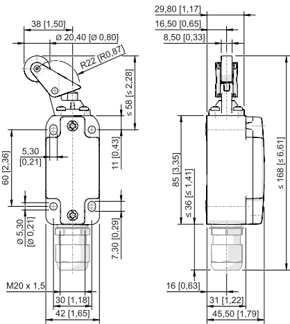
Rollenhebel 8070/2-5-WPH-U60
