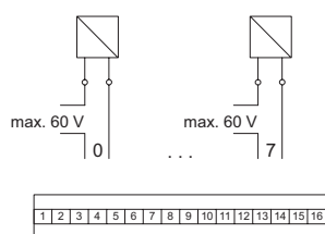
9477/12-08-12 connection diagram
