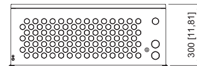
1 x BusRail for 10 slots Item no. 244144
