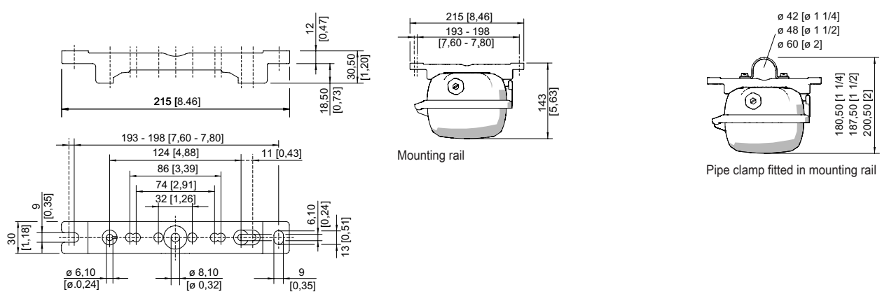
Mounting rail
