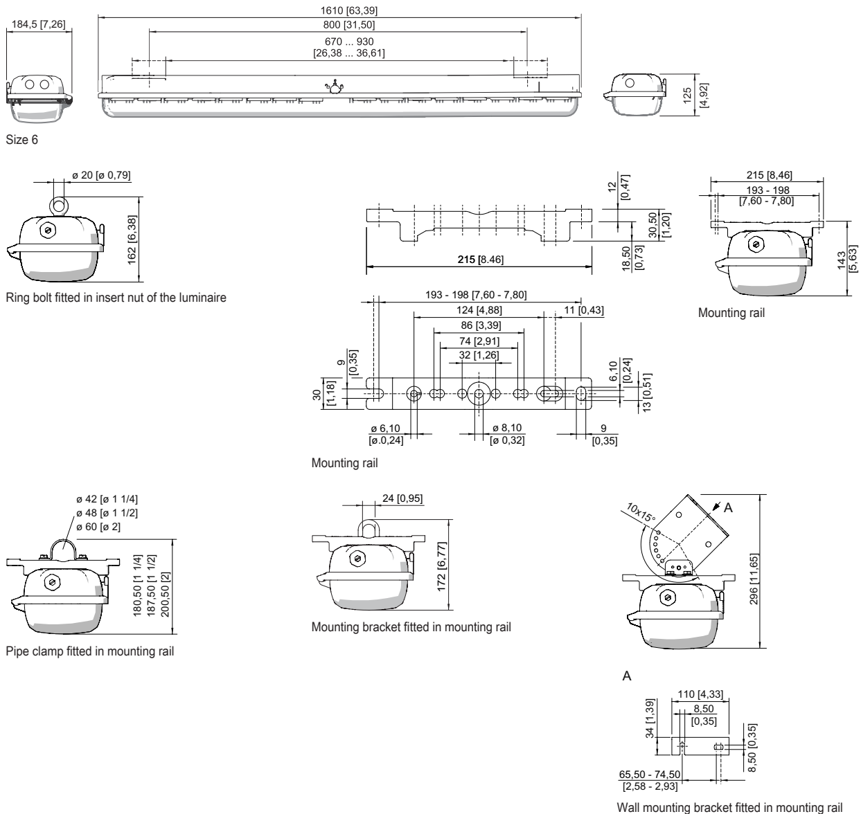
Wall mounting bracket fitted in mounting rail
