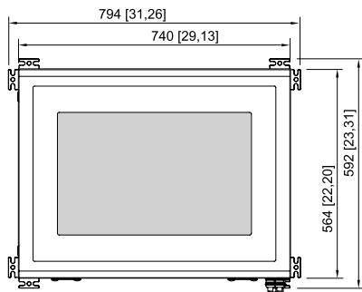
Operator Station FR enclosure, wall mounting
