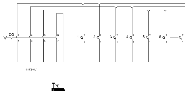
Circuit diagram 8146/5-ExV-...1P-D; 8264/5-ExV-...1P-D
