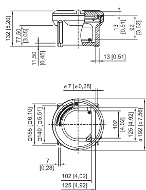
Size 2 enclosure without sight glass
