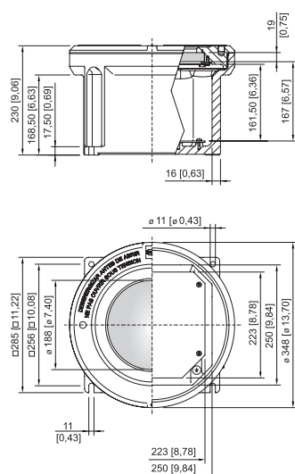
Size 5 enclosure with sight glass
