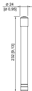
Antenna type 9790/1-2458-NTM-53
