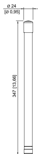
Antenna type 9790/1-0826-NTM-02
