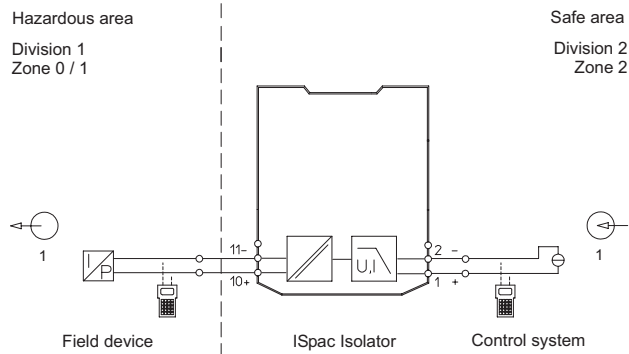
Connection diagram 9167/1
