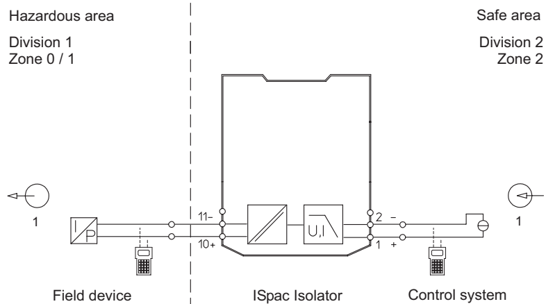
Connection diagram 9167/1
