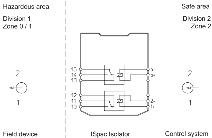
Connection diagram 9172/21-11-00
