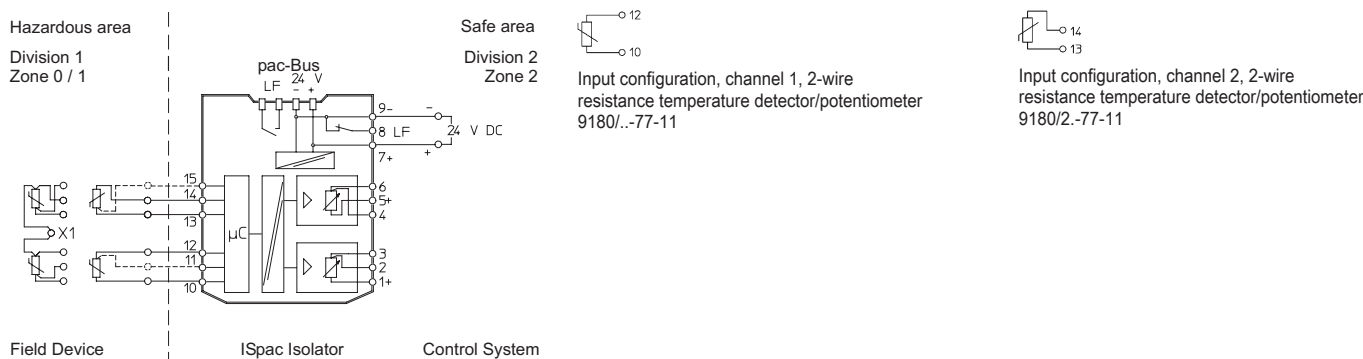
9180/2.-77-11 connection diagram
