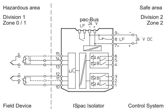
Connection diagram 9182/20-50-12
