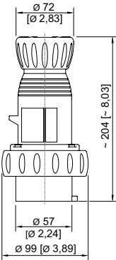
4-pole plug
