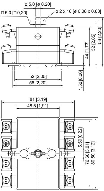
Load and motor switches Series 8006/4, 1-pole and 2-pole
