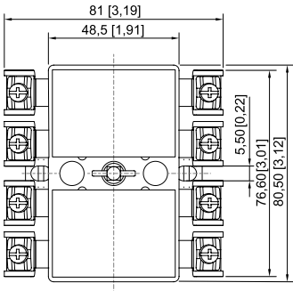
Load and motor switches Series 8006/4, 1-pole and 2-pole
