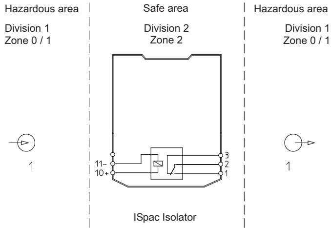
Connection diagram 9172/12-11-00
