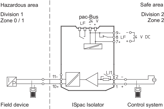
Connection diagram 9165/16-11-11
