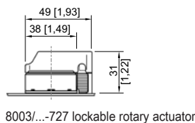
8003/...-727 lockable rotary actuator
