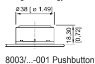
8003/...-001 Pushbutton
