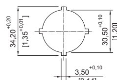
Punch pattern
