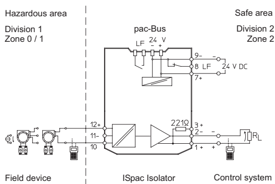
Connection diagram 9160/13-11-13
