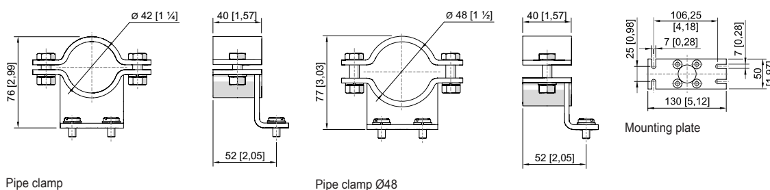
Pipe clamp
