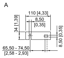
Wall mounting bracket fitted in mounting rail
