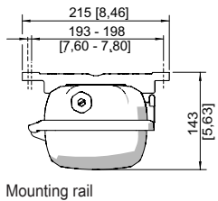
Mounting rail
