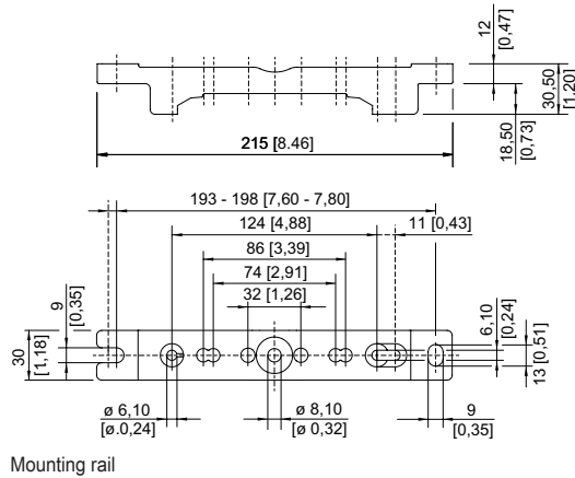
Mounting rail
