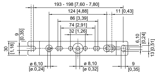
Mounting rail
