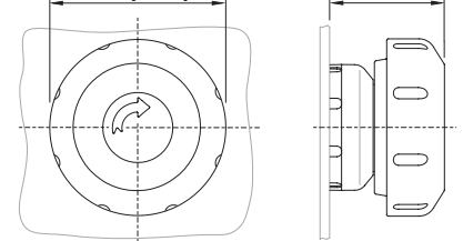
8602/3-015 red/yellow mushroom stay-put button Actuator with axial actuation
