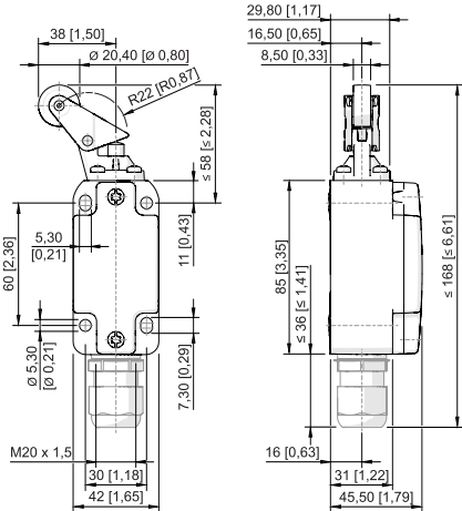
Roller lever 8070/2-2-WPH-U60
