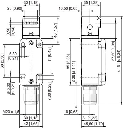
Safety switch 8070/2-3-AZ-U50
