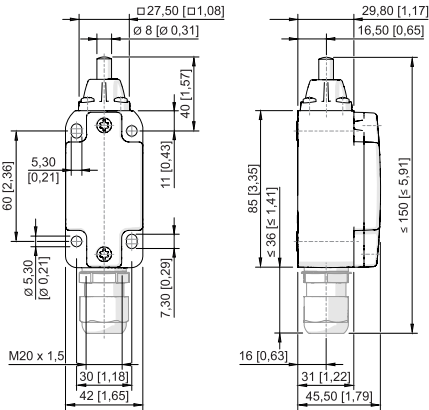
Domed plunger 8070/2-5-W-U60
