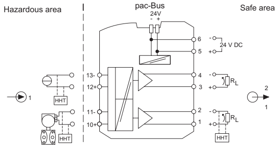
9260/19-11-10 connection diagram
