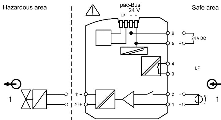
Connection diagram 9275/10-21-25-11
