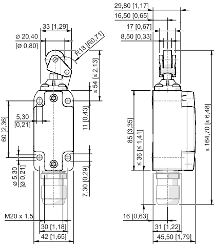
Roller lever 8070/2-5-WH-U60
