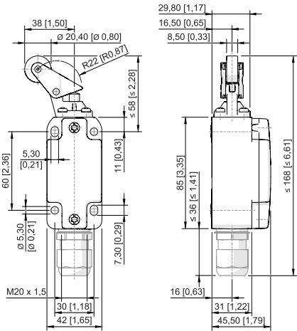
Roller lever 8070/2-5-WPH-U60
