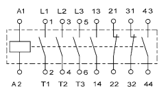
Contact arrangements
