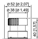
8003/...-010, 8003/...-012 Mushroom stay-put button Ø 38 mm
