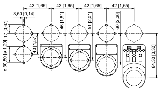
8003/...-008 key-operated switch
