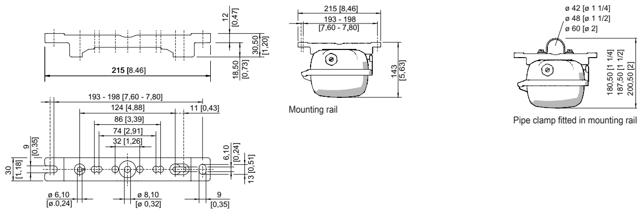
Mounting rail
