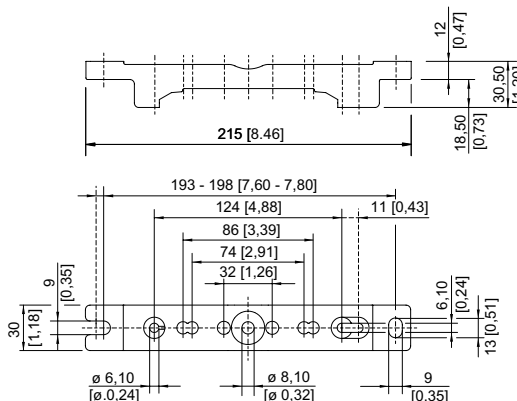
Mounting rail
