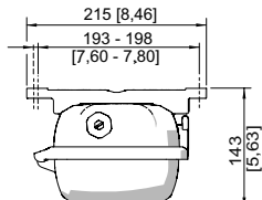
Mounting rail
