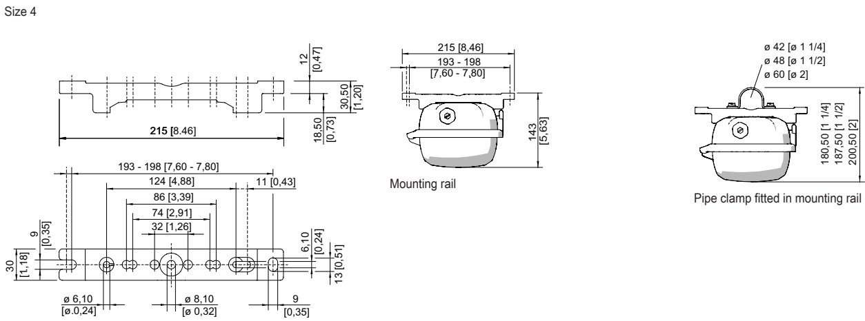
Mounting rail
