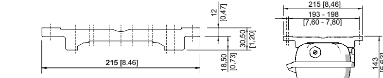
Mounting rail
