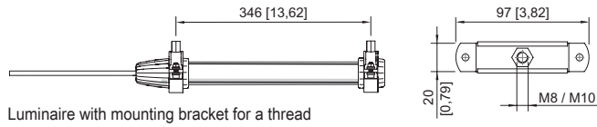
Luminaire with mounting bracket for a thread
