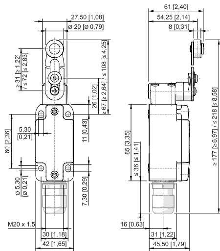
Swivelling lever 8070/2.-DS-U60
